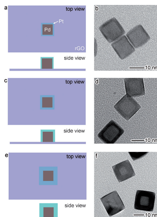
Figure 2. Schematic illustrations and TEM images for a, b) Pt-Pd-rGO I; c, d) Pt-Pd-rGO II; and e, f) Pt-Pd-rGO III hybrid structures with tunable Pt thickness.
